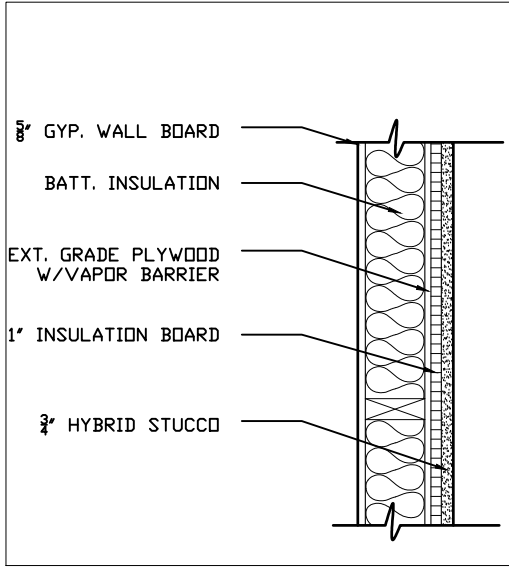
003 Wall Section 3/4"=1'-0"
