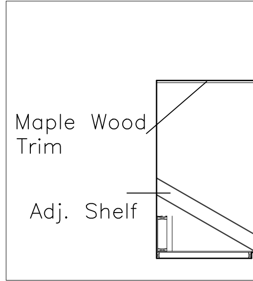
004 Base Cabinet 1/2"-1'-0"
